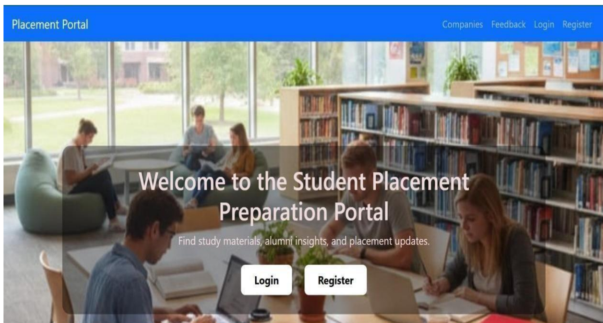
Fig 5.1.1 Landing Page
