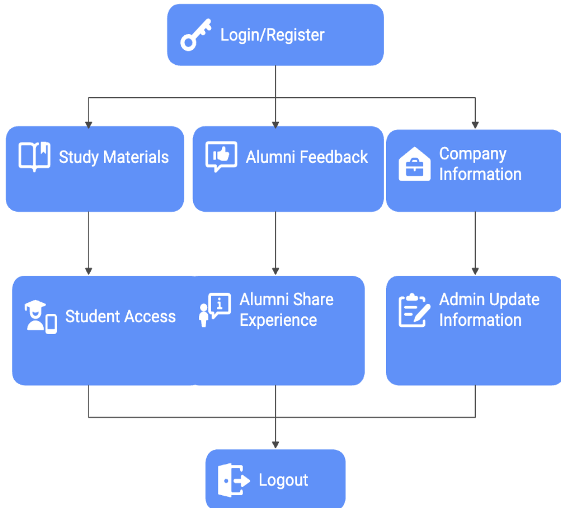
Fig 2.1 : System Architecture
